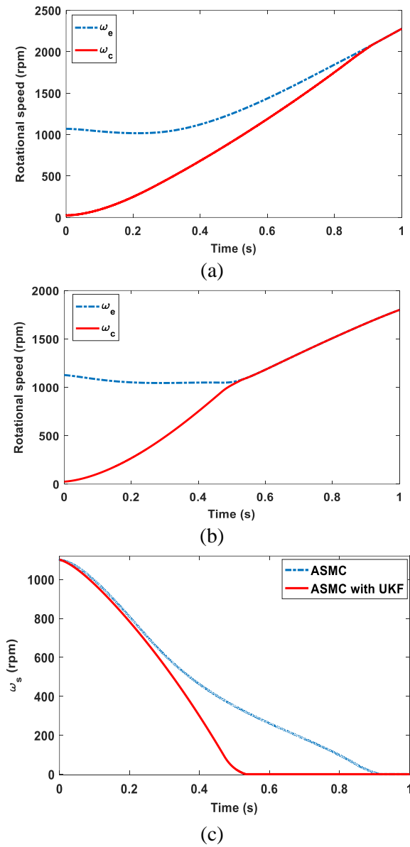
Figure 14: Slip speed during clutch engagement for the ASMC method in comparison with the ASMC system with \mu estimator in case of 30% uncertainties in the road friction coefficient (a): \omega_e and \omega_c of ASMC system, (b): \omega_e and \omega_c of ASMC system with \mu estimator, (C): Clutch slip speed
